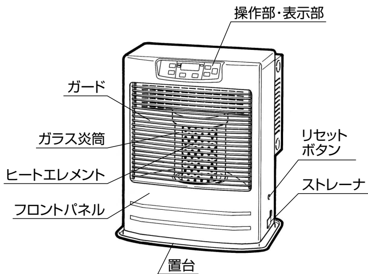
外観図 FR-S45C・FR-S55C
